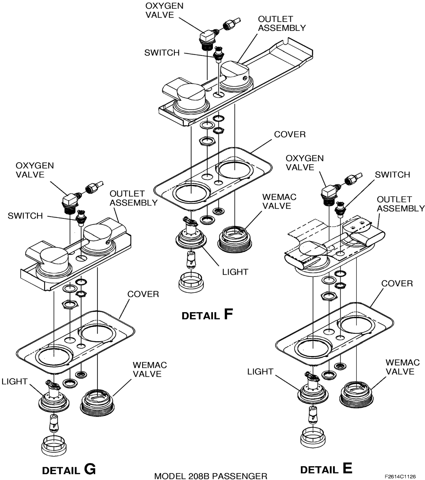
Figure 201 : Sheet 8 : Cabin Air Ventilation System
